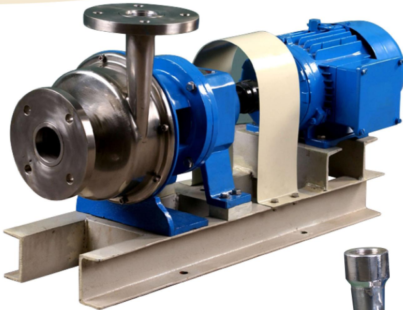
SS 304/316 Coupled Centrifugal
